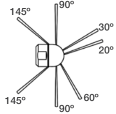
UNIVERSAL 044 7 Ports: 1 @ 20°, 1 @ 30° 1 @ 60°, 2 @ 90°, 2 @ 145°
