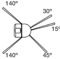
UNPLUGGER 043 5 Ports: 1 @ 15°, 1 @ 30° 1 @ 45°, 2 @ 145°
